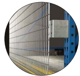
Heavy-Duty Brackets Ensure Panel Stability
